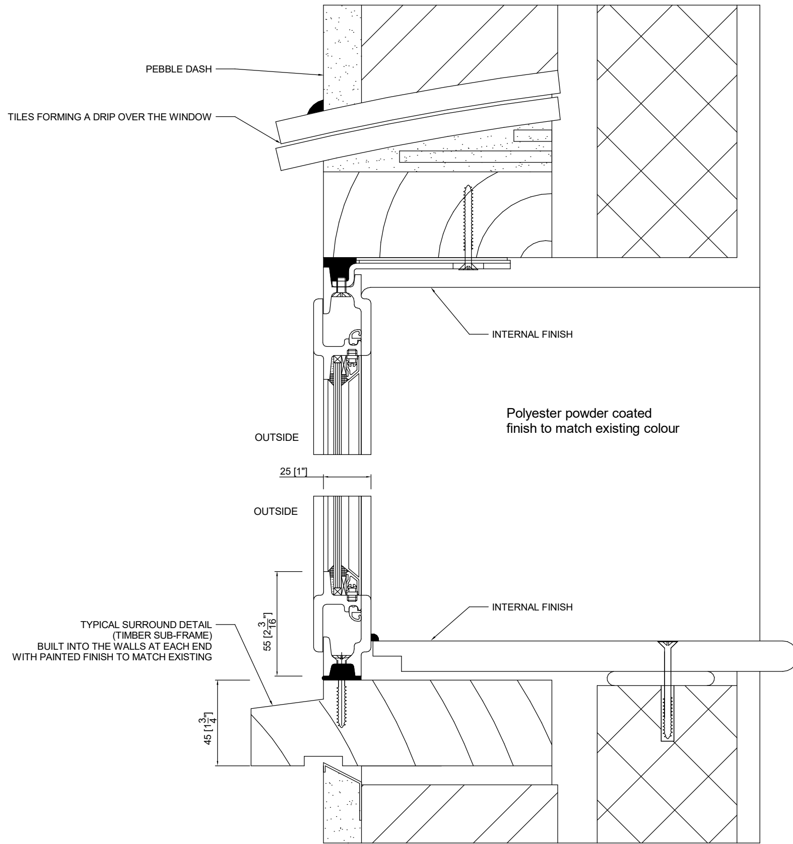
TYPICAL SURROUND DETAIL
