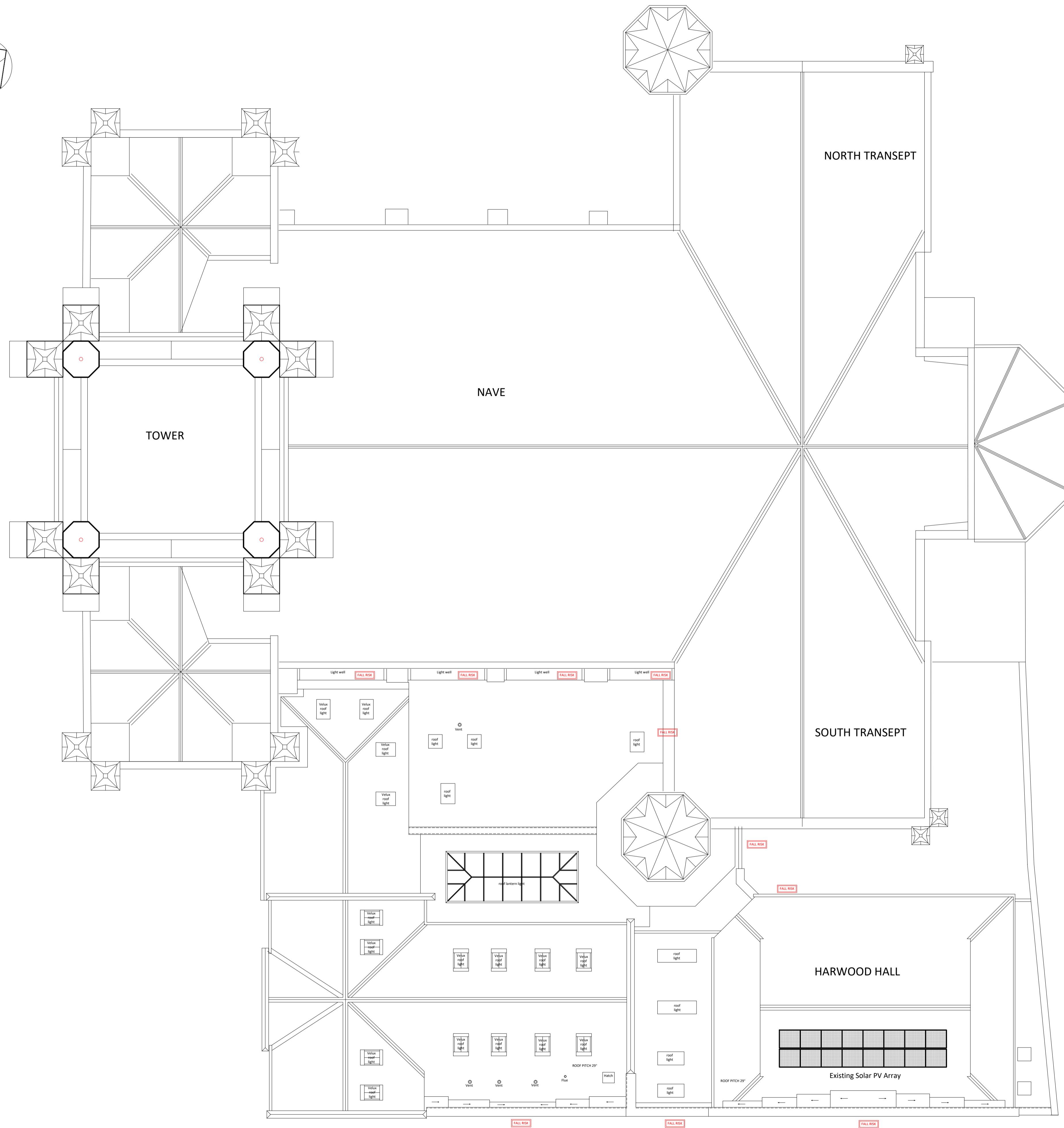
CHURCH AND PARISH HALLS: EXISTING ROOF PLAN, INCLUDING EXISTING SOLAR PV ARRAY INSTALLATION TO HARWOOD HALL ROOF CHRIST CHURCH, MALVERN ROAD, CHELTENHAM, GLOUCESTER DIOCESE
