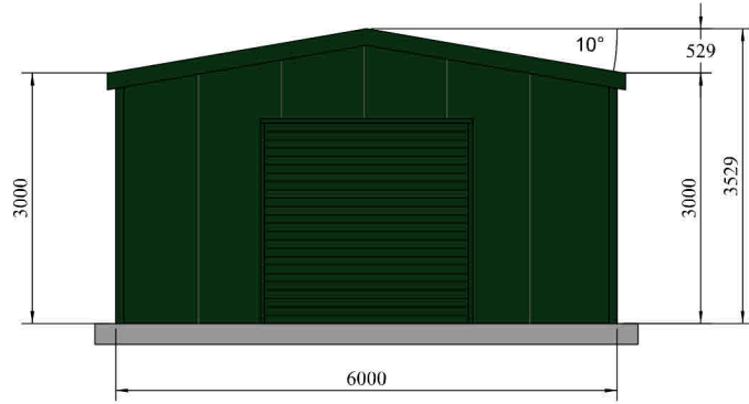
Front Elevation (External)
