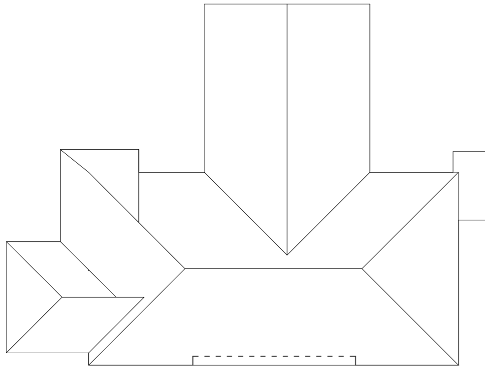
ROOF PLAN 1:200 existing
