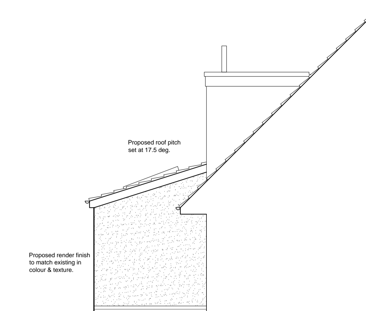
BOUNDARY ELEVATION
