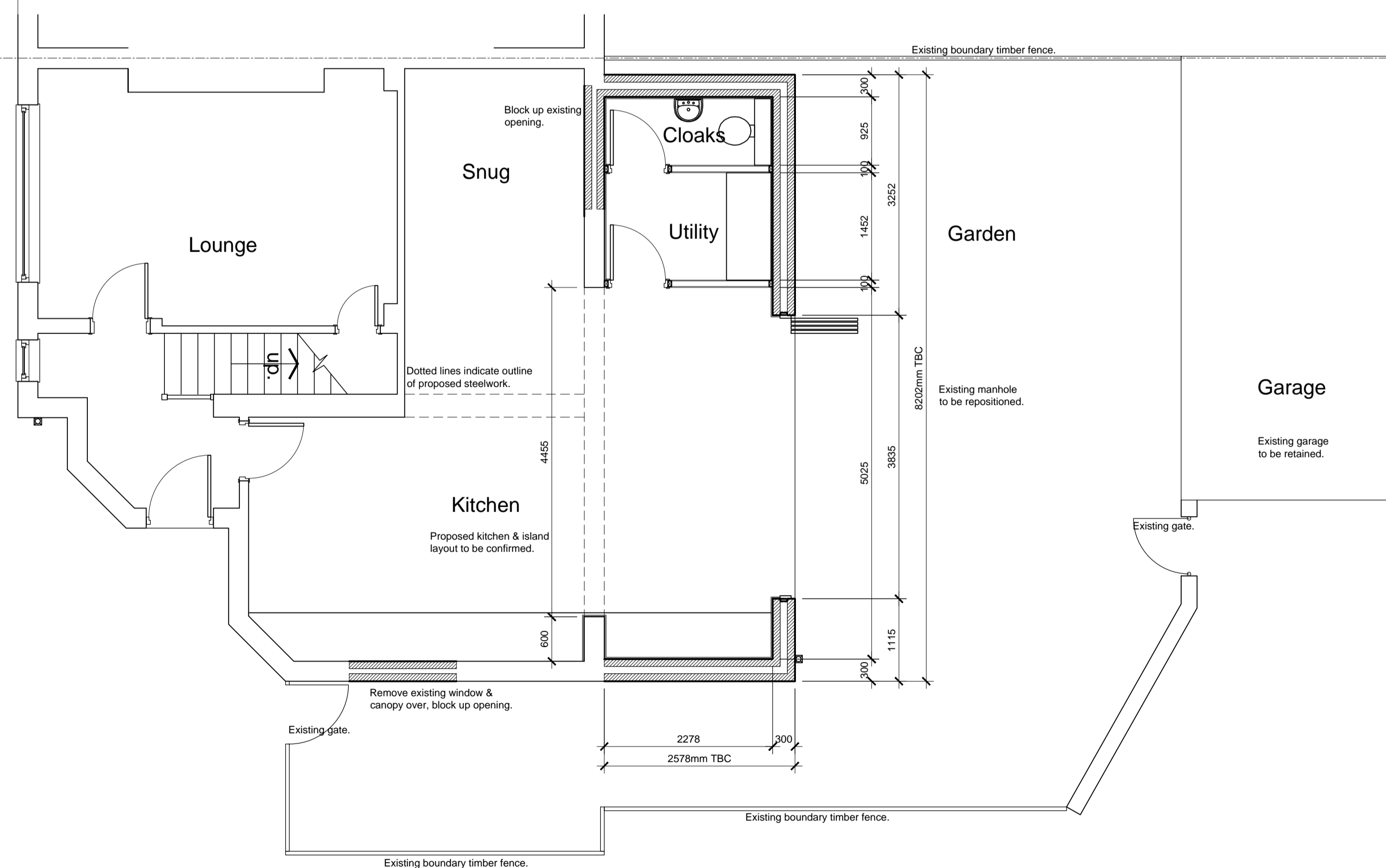
GROUND FLOOR LAYOUT
