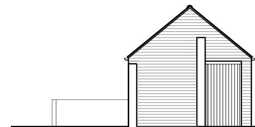
Existing West Elevation 1:100
