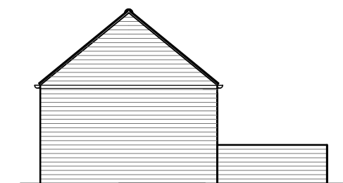
Existing East Elevation 1:100
