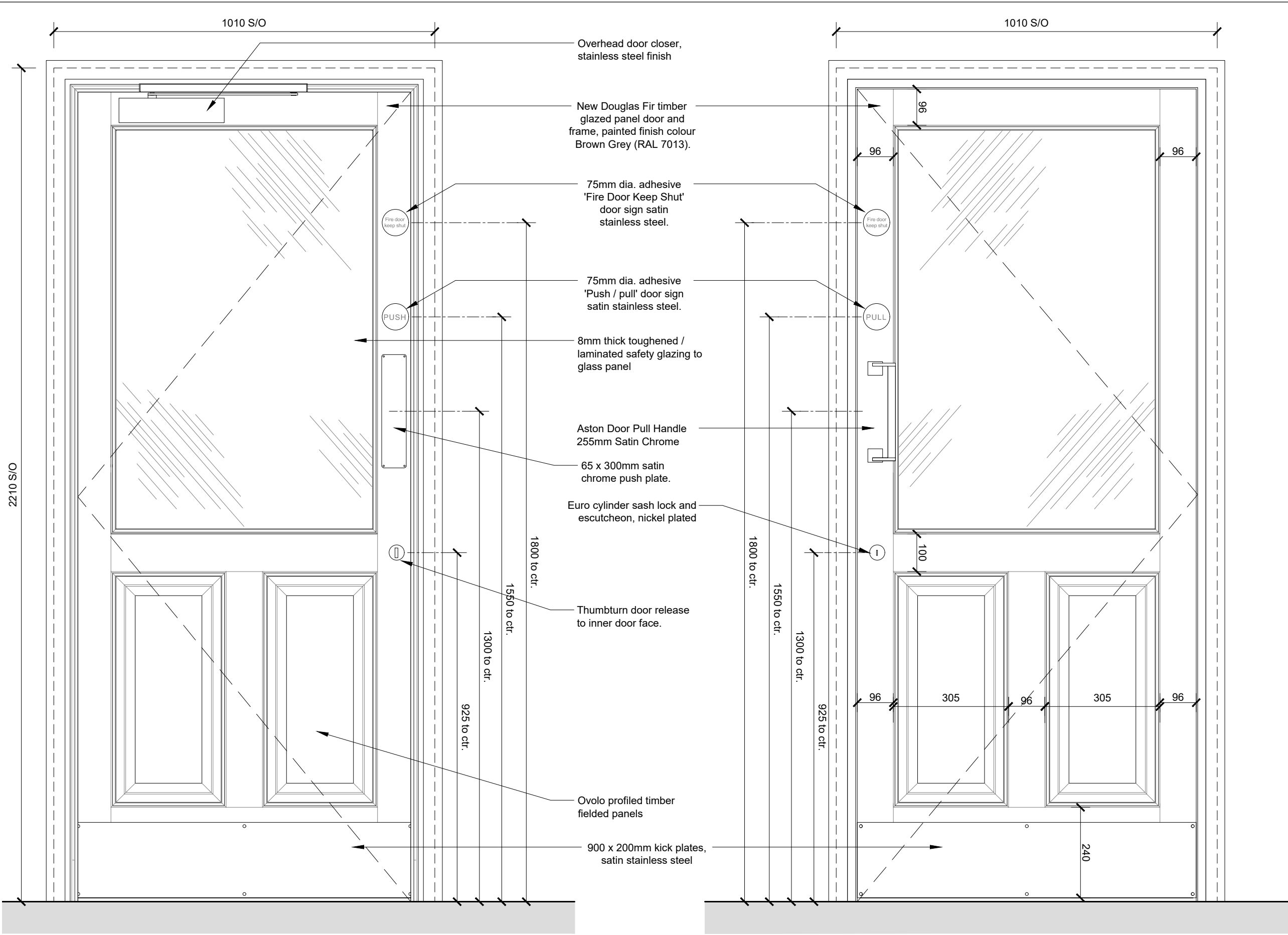
PROPOSED REAR ELEVATION 1:10 @ A3
