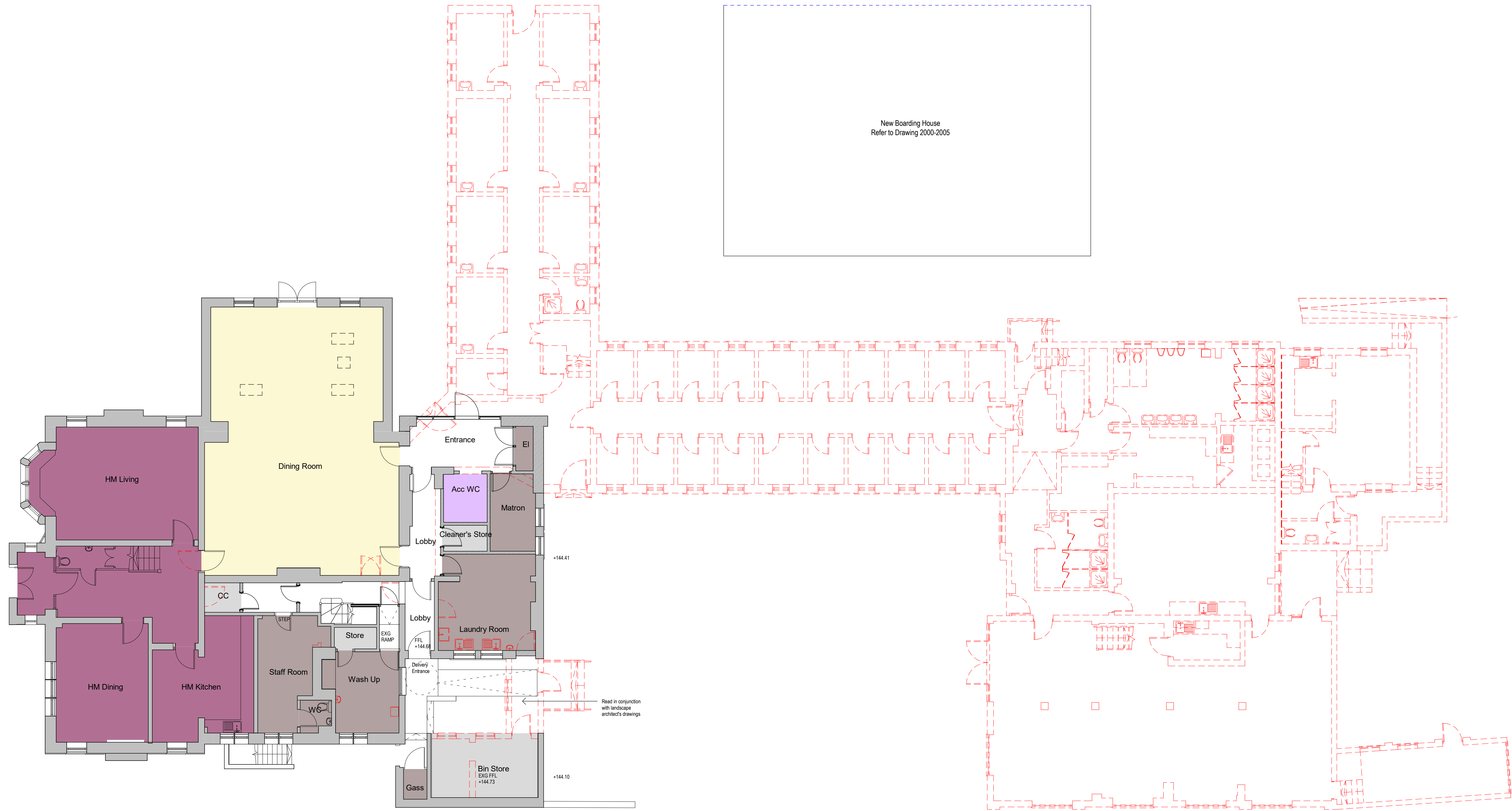
1 Proposed Ground Floor Plan 2020 1 : 100
