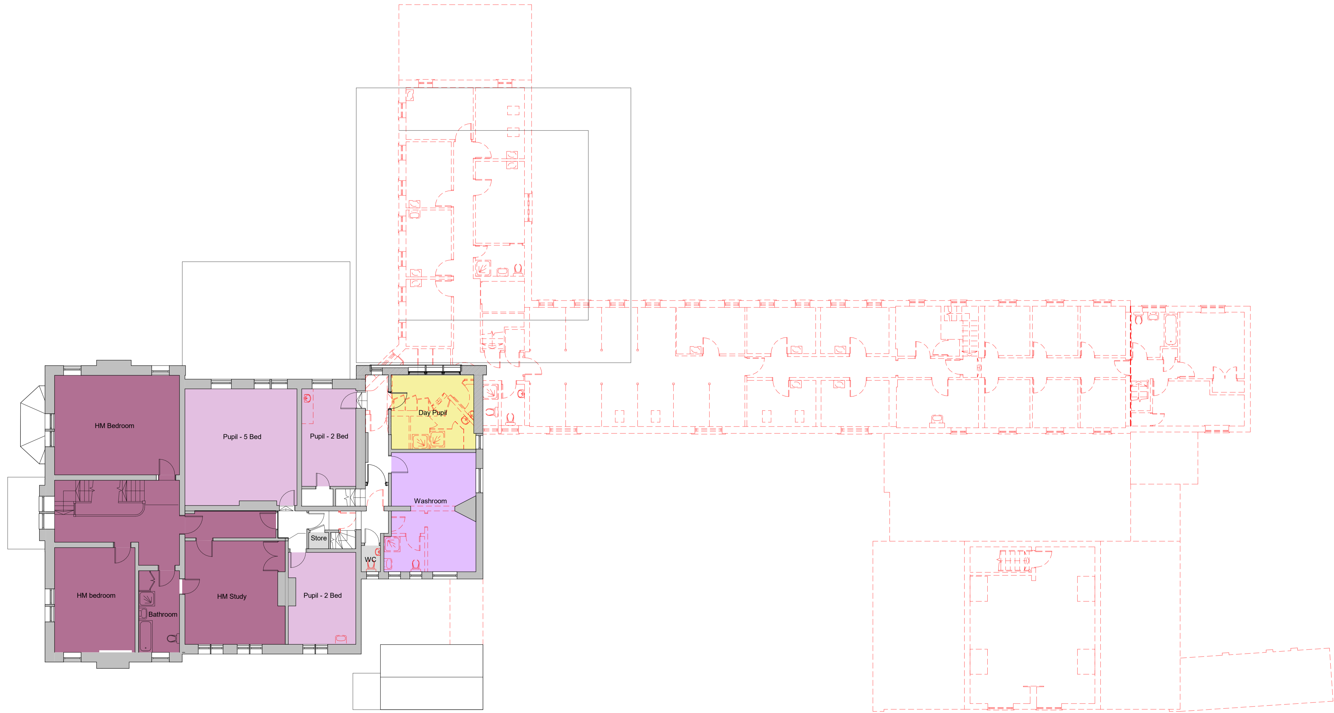
1 Proposed First Floor Plan 2021 1 : 100
