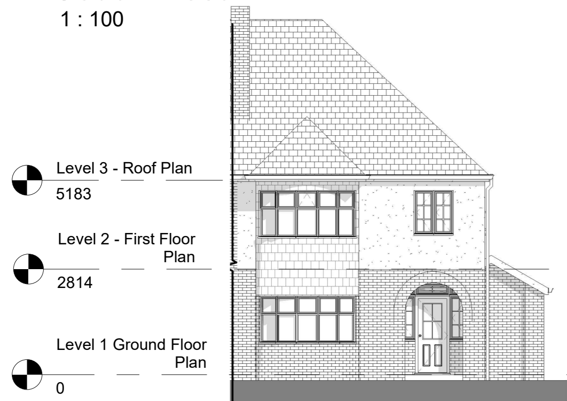
North East 1 : 100
