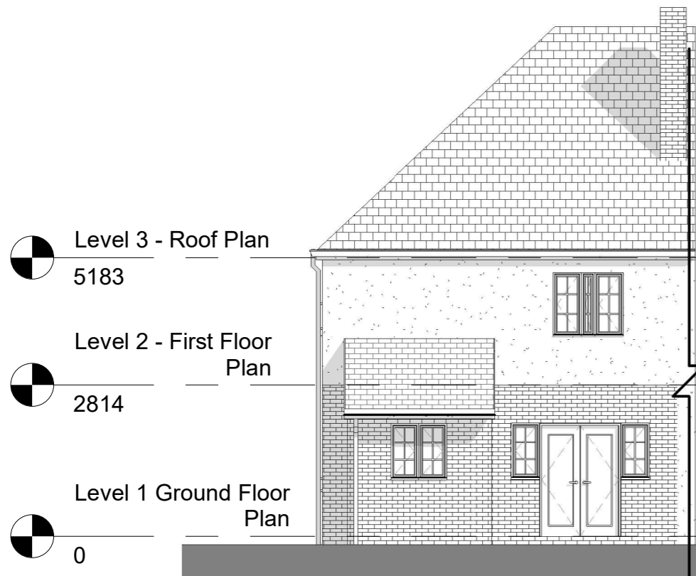
South West 1 : 100
