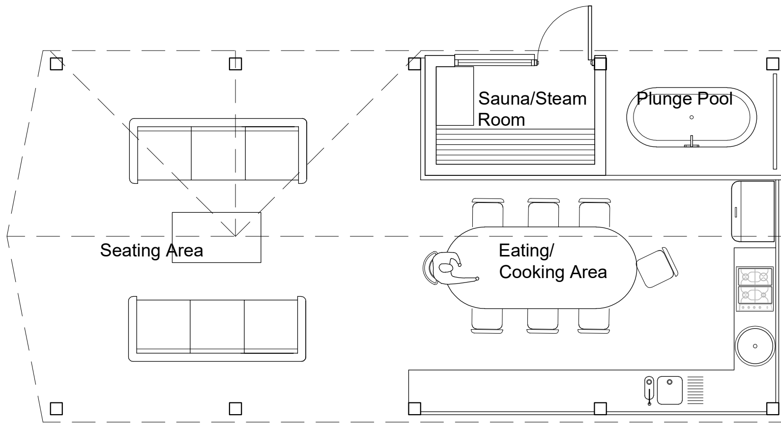
KITCHEN PLAN
