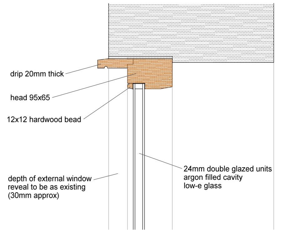
DETAIL 2 1:5
