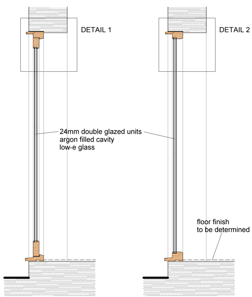
SECTION 1:20
