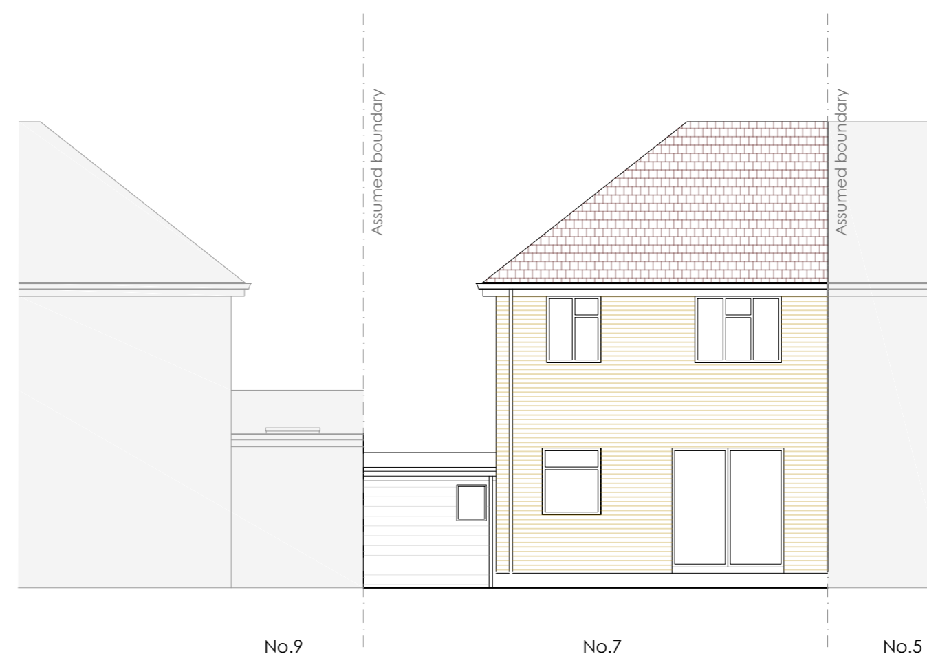
4 Existing Rear Elevation
