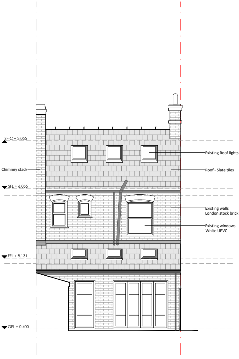
REAR ELEVATION
