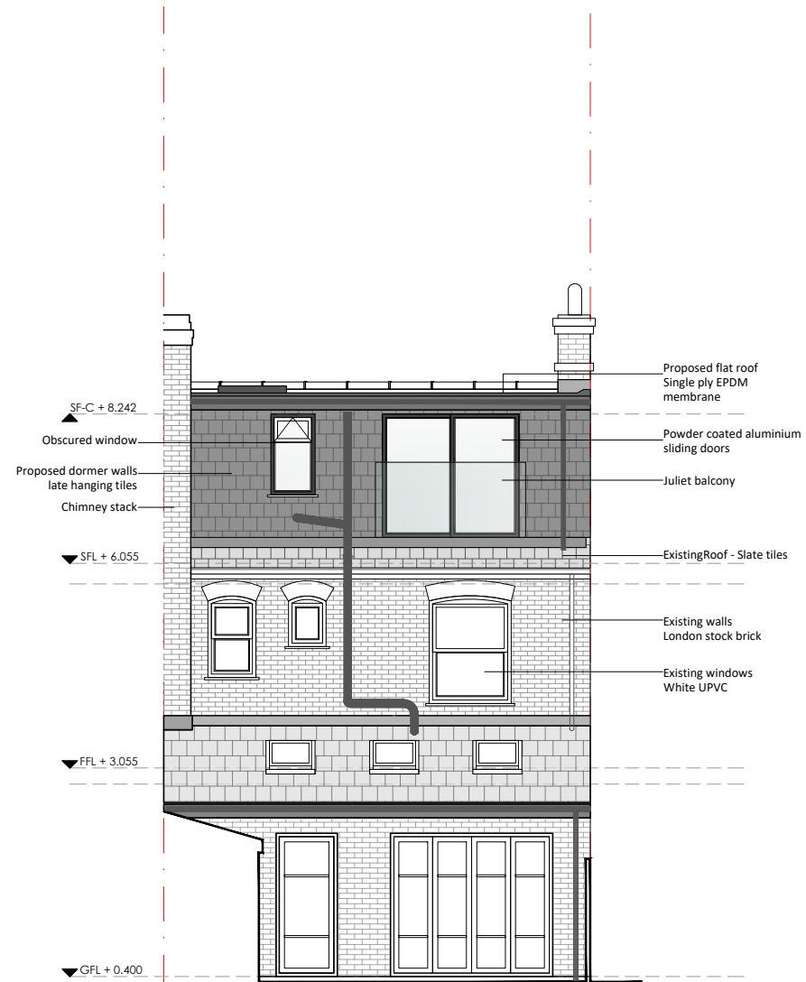
REAR ELEVATION
