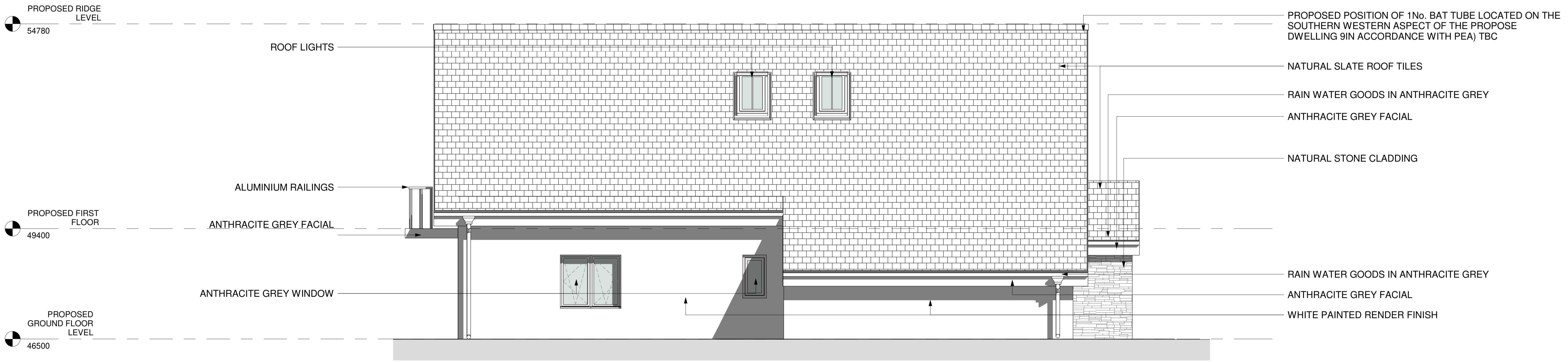
2 PROPOSED ELEVATION NW 1 : 50
