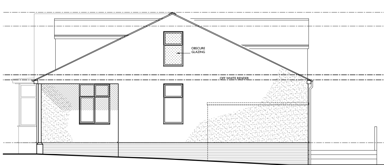
Proposed Section BB / Side Elevation
