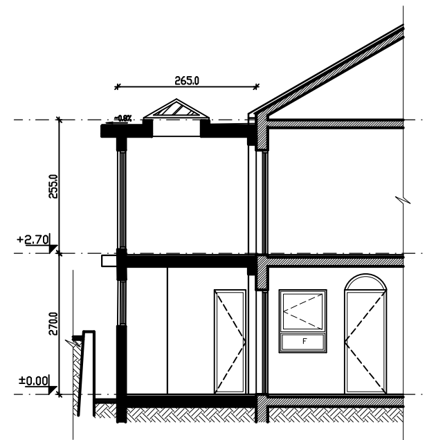
Section 1:100
