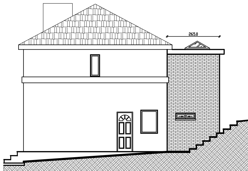
PROPOSED ELEVATION: SOUTH
