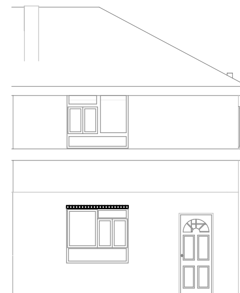
BVN.03.3 E-09 EXISTING ELEVATION: WEST
