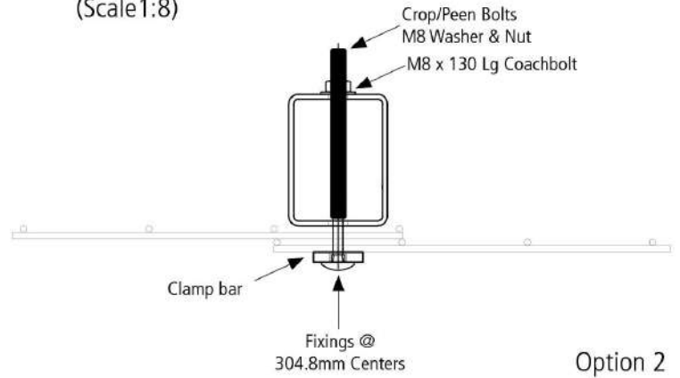
Mesh Clamp Detail (Scale 1:8)
