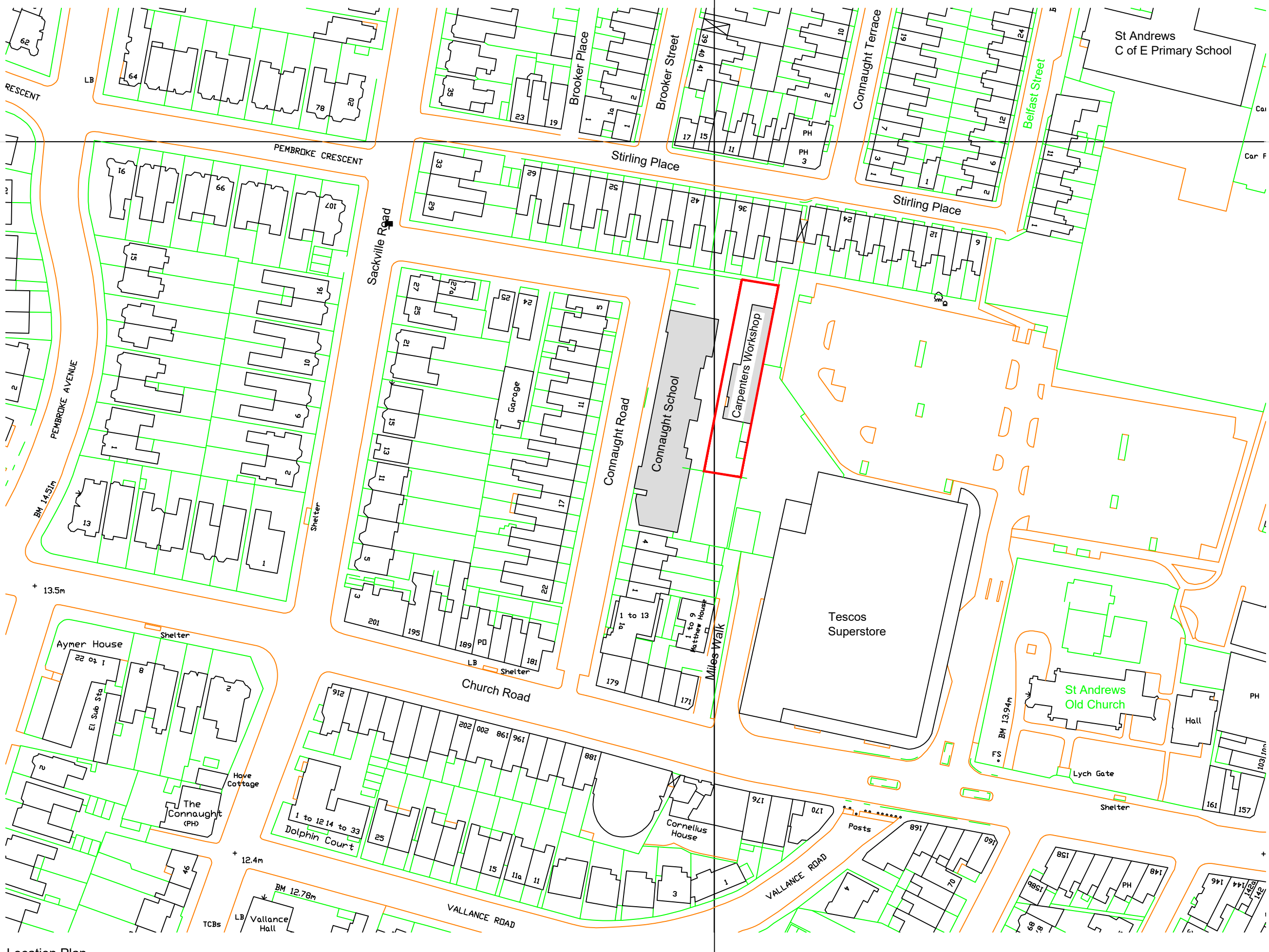
Location Plan As Existing Scale 1:1250
