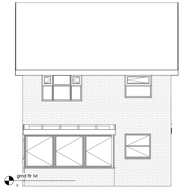
Existing Elevation-Rear
