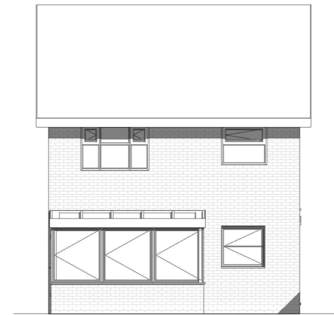
Proposed Elevation-Rear
