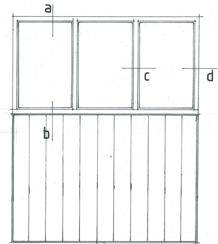
timber paneling & fixed window 1:20
