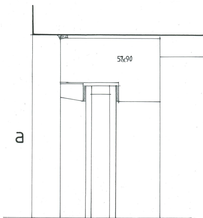
window frame details 1:2
