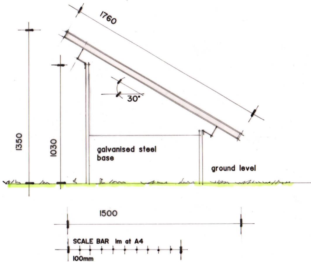
FIG 1: DETAIL SECTION
