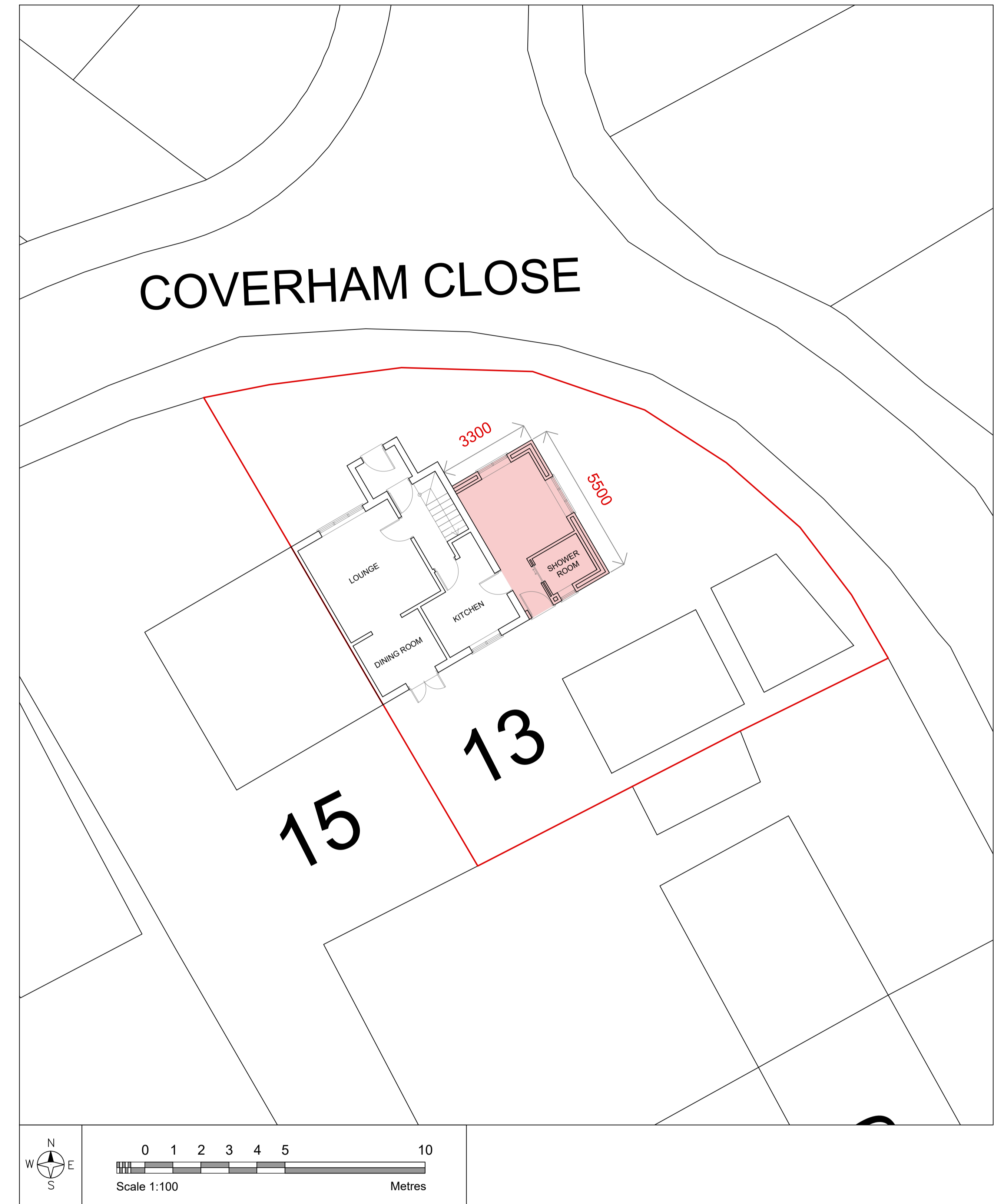
Block plan - Scale 1:100 - Proposed
