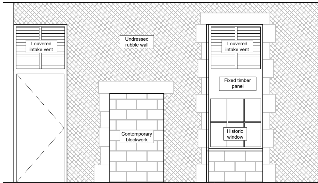
Existing Elevation A (1:50)
