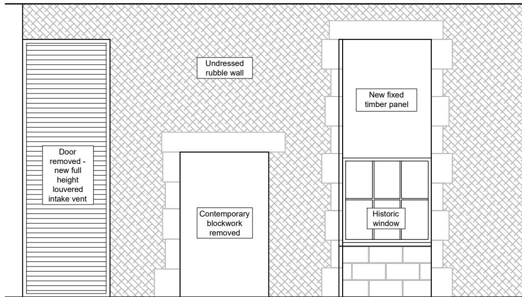
Proposed Elevation A (1:50)
