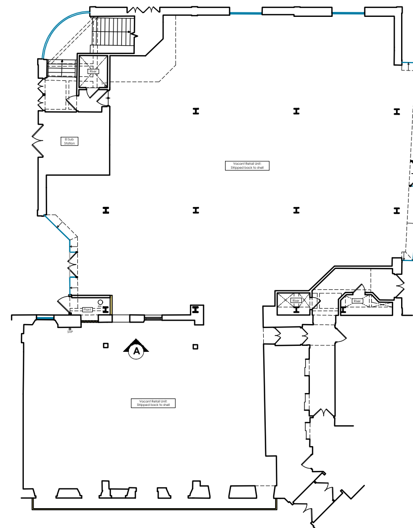
Reference Plan (1:250)
