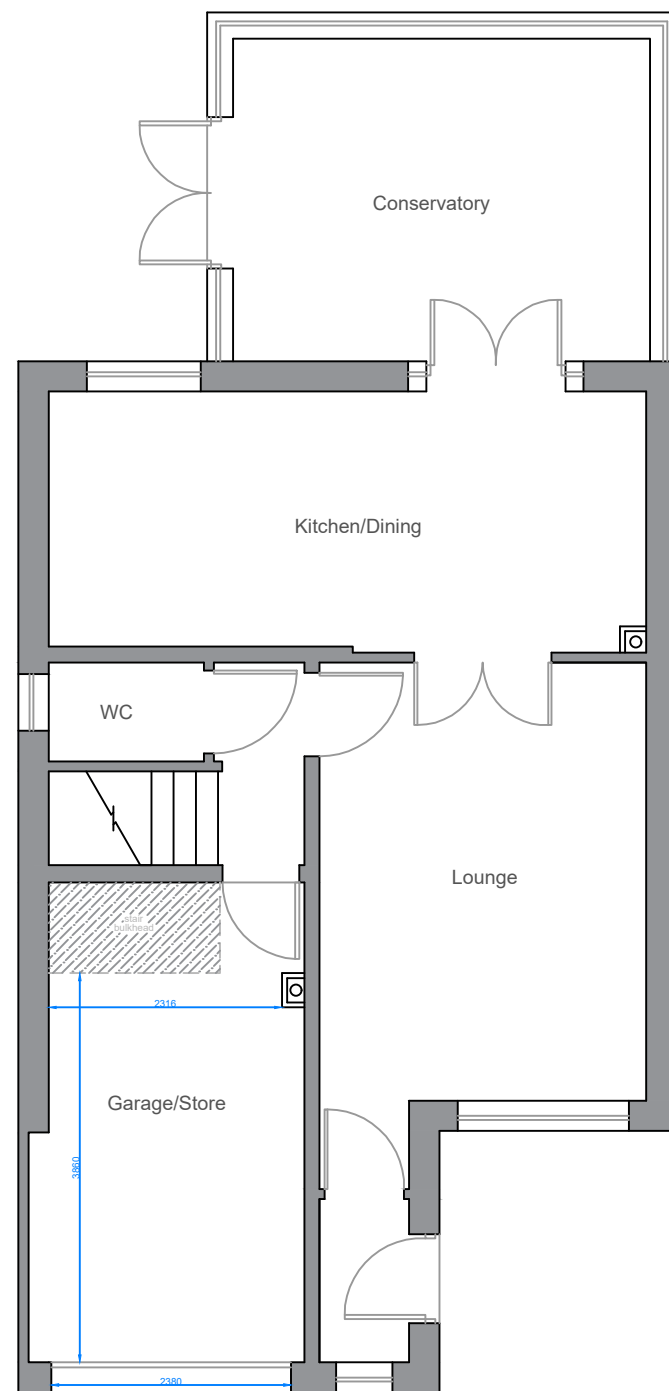
Existing Ground Floor Layout
