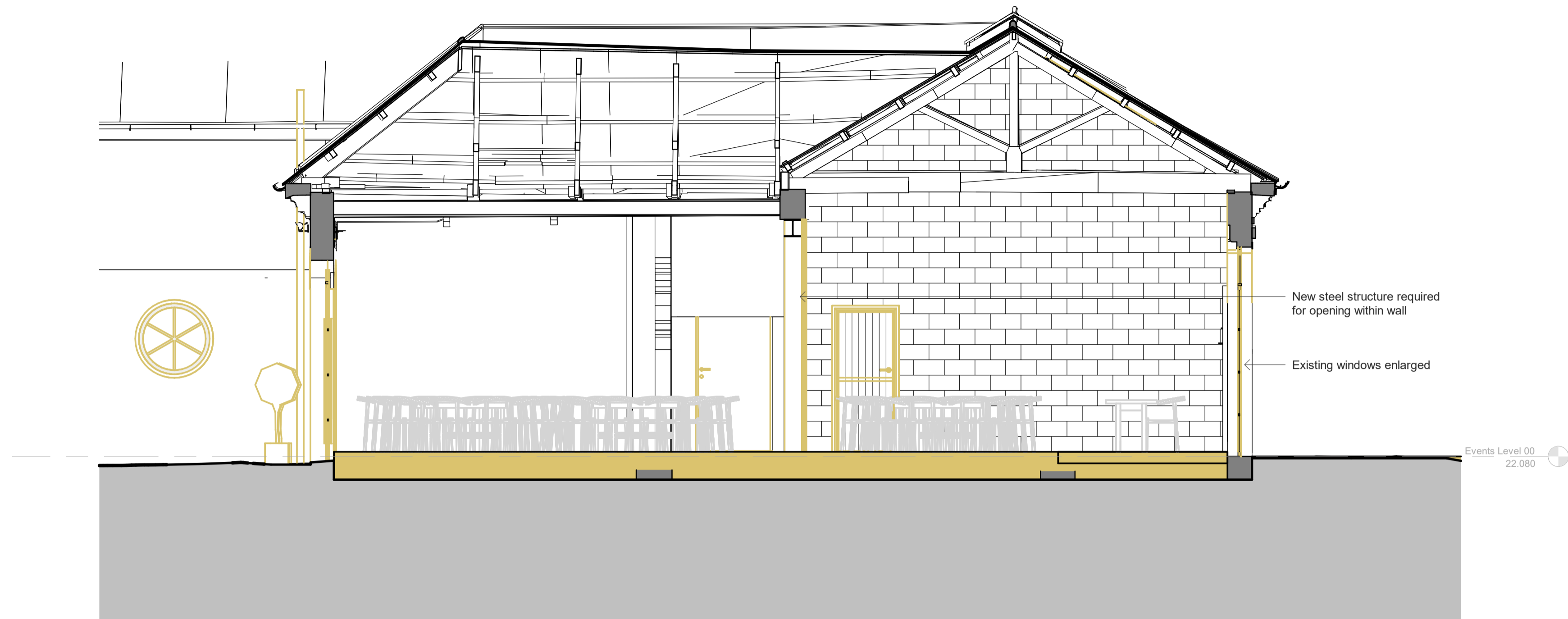
Section 10 - Proposed 1 : 50
