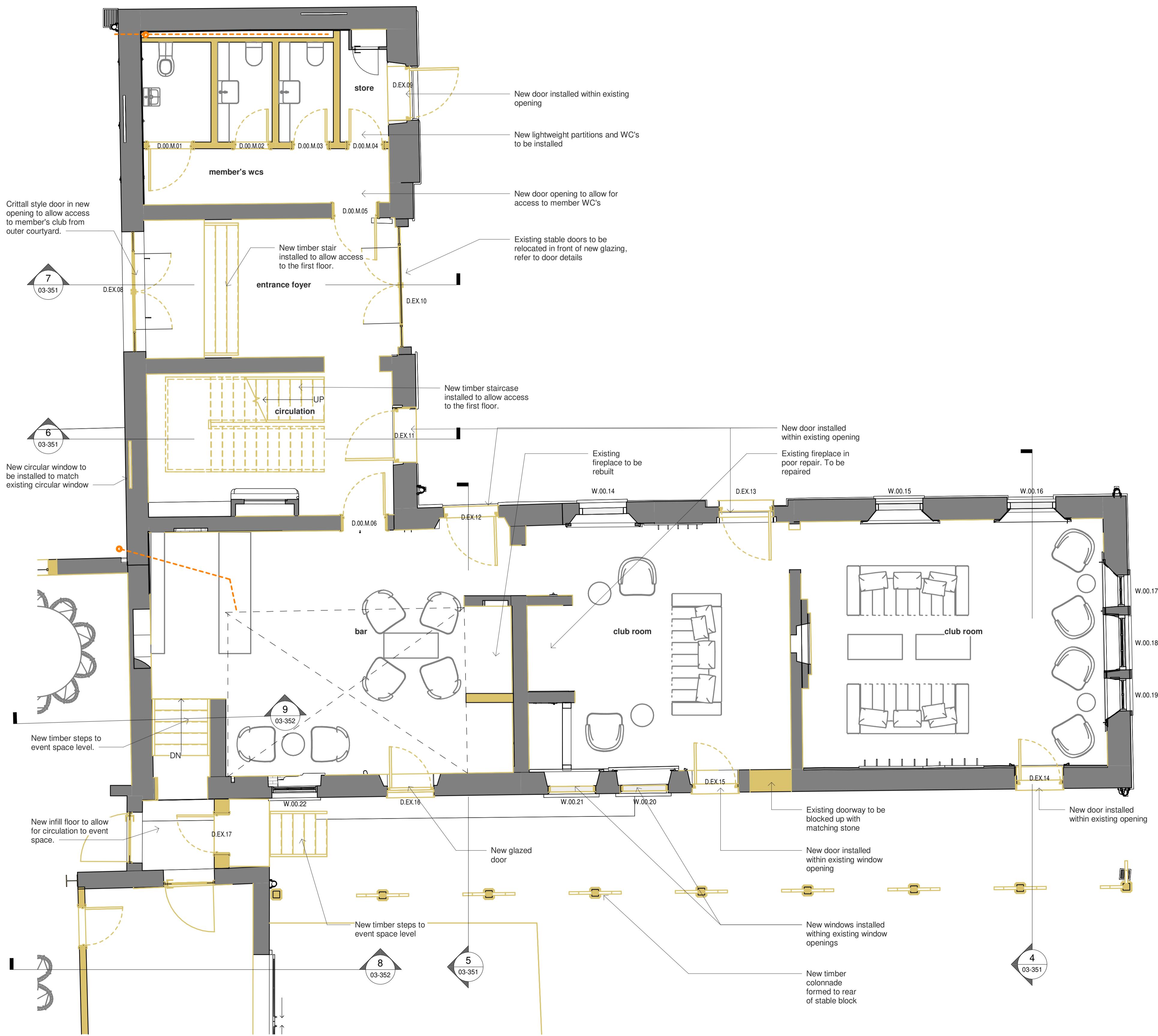
Member's Club - Ground Floor Proposed 1 : 50
