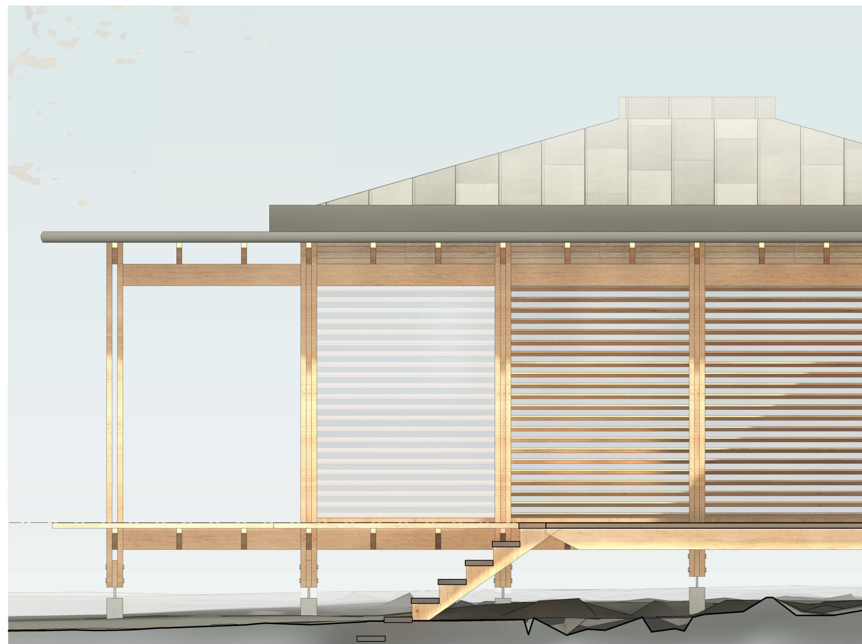
Section 01 - Proposed - Callout 2 1 : 20
