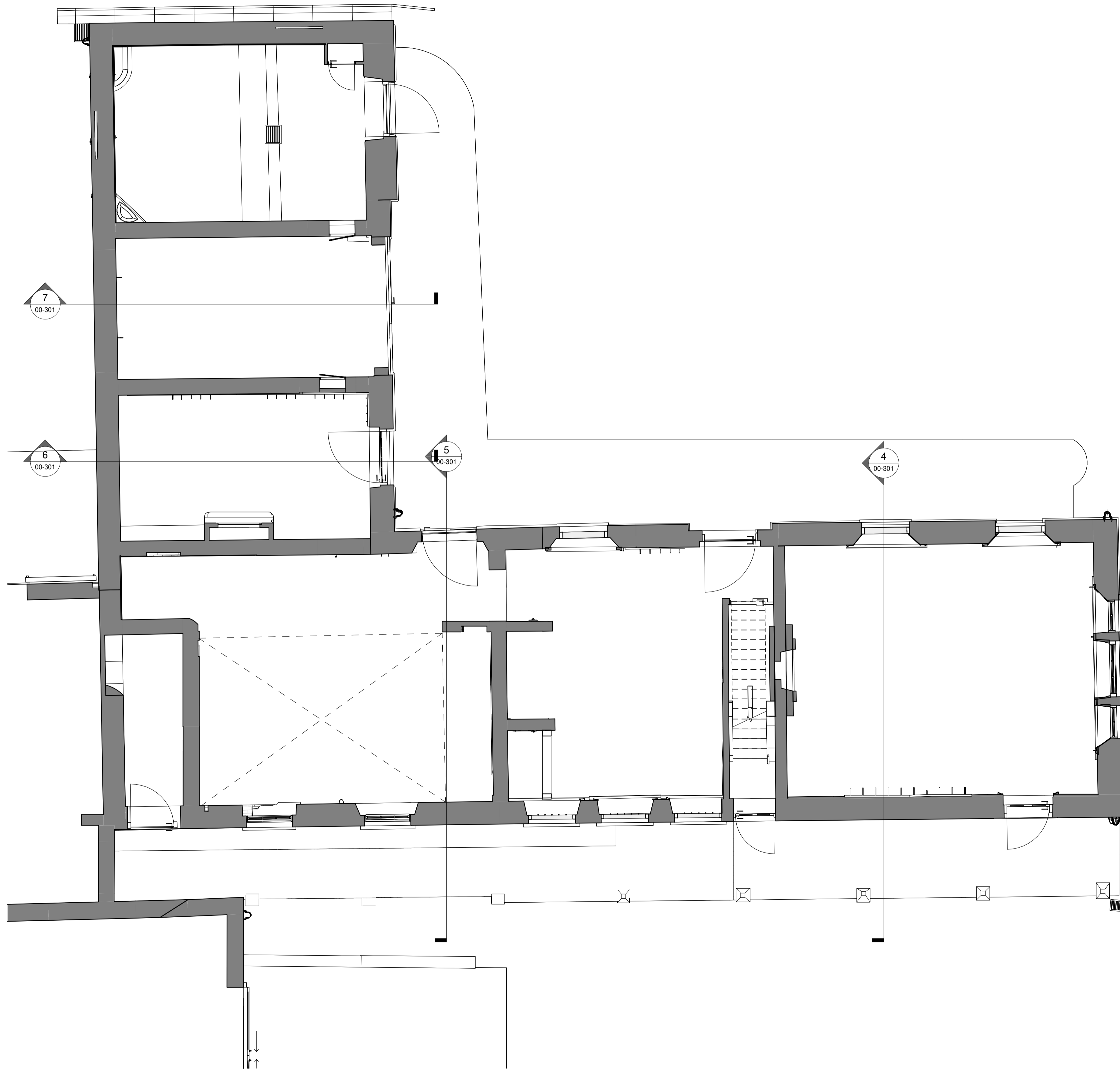
Member's Club - Ground Floor Existing 1 : 50
