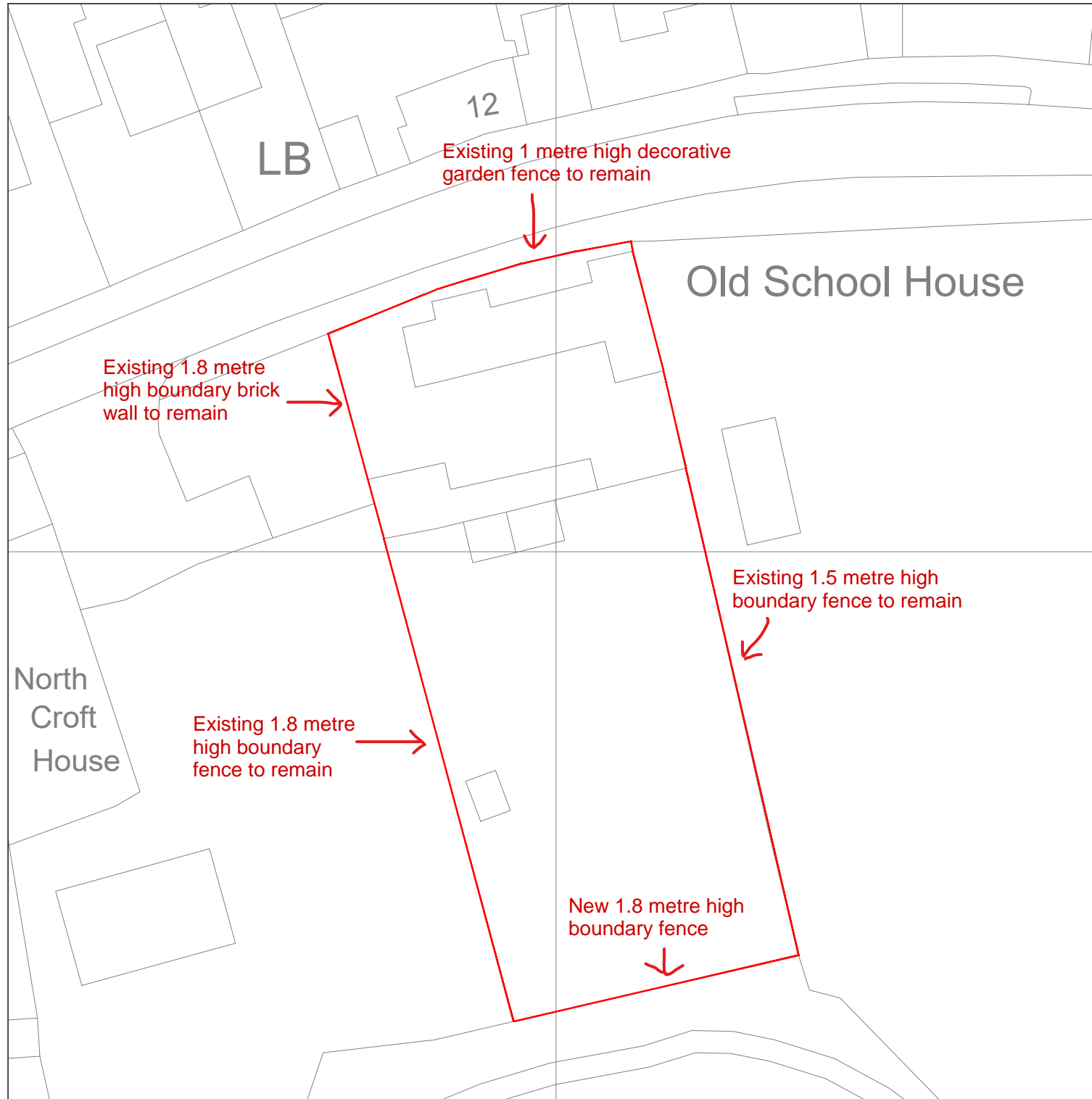
BLOCK PLAN 1:500
