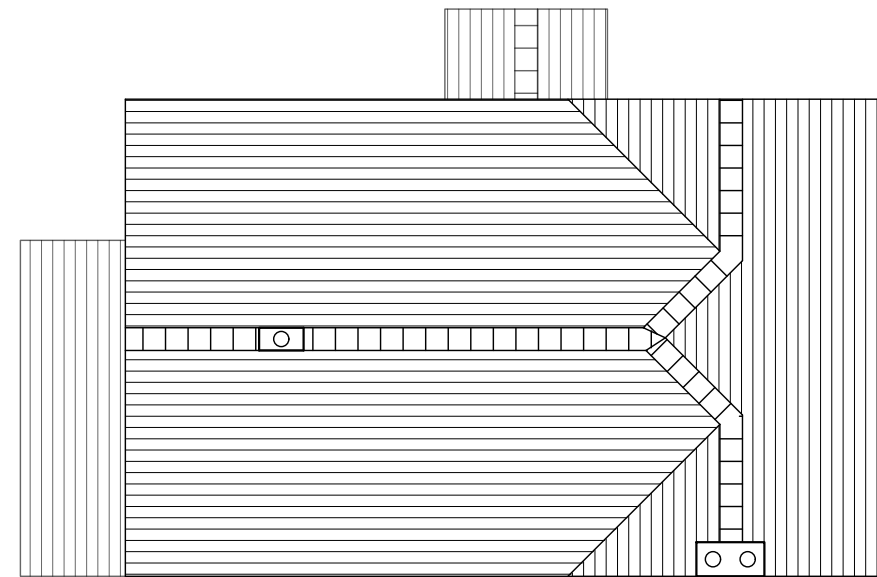
Roof Plan 1:100
