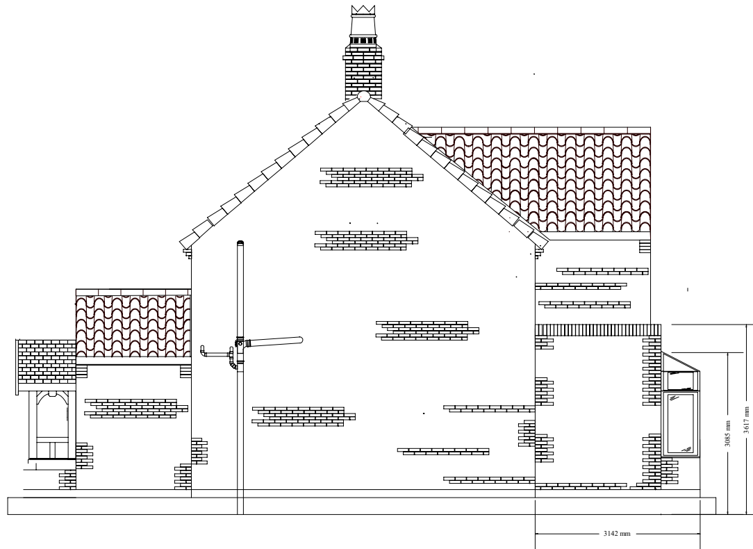
Revised North Elevation for Proposed Alterations to the rear of Endlich, Main Street, Carlton on Trent Scale 1:100 Date 09/2/2024
