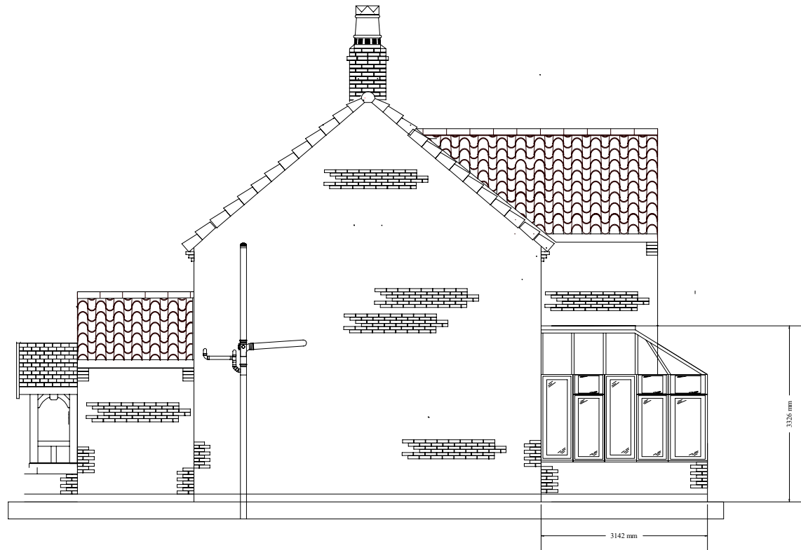
Existing North elevation for Proposed Alterations to the rear of Endlich, Main Street, Carlton on Trent Scale 1:100 Date 09/02/2024
