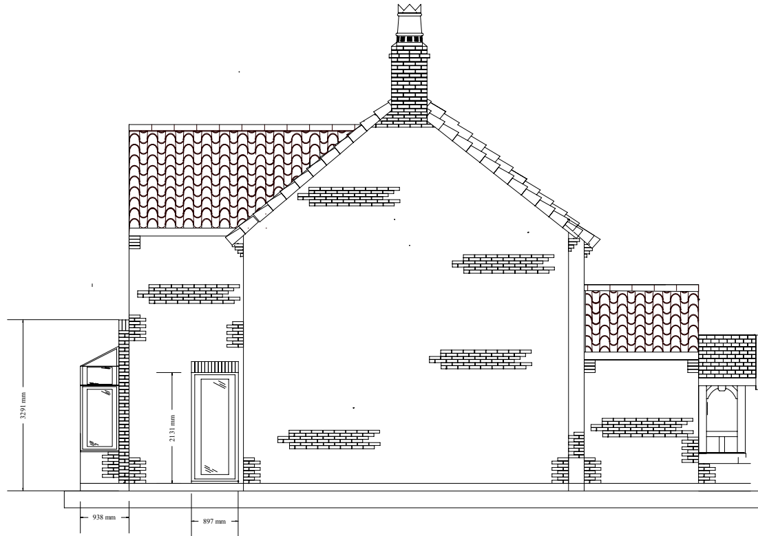
Revised South Elevation for Proposed Alterations to the rear of Endlich, Main Street, Carlton on Trent Scale 1:100 Date 09/2/2024
