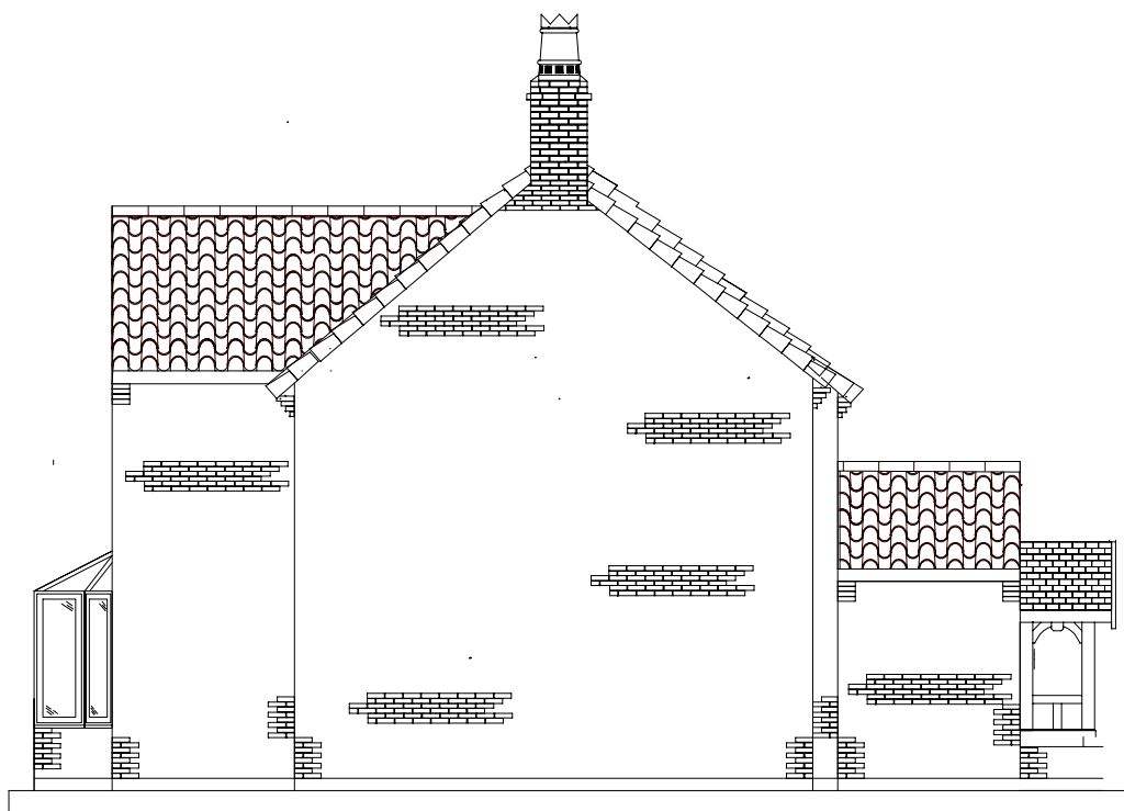
Existing South elevation for Proposed Alterations to the rear of Endlich, Main Street, Carlton on Trent Scale 1:100 Date 09/02/2024
