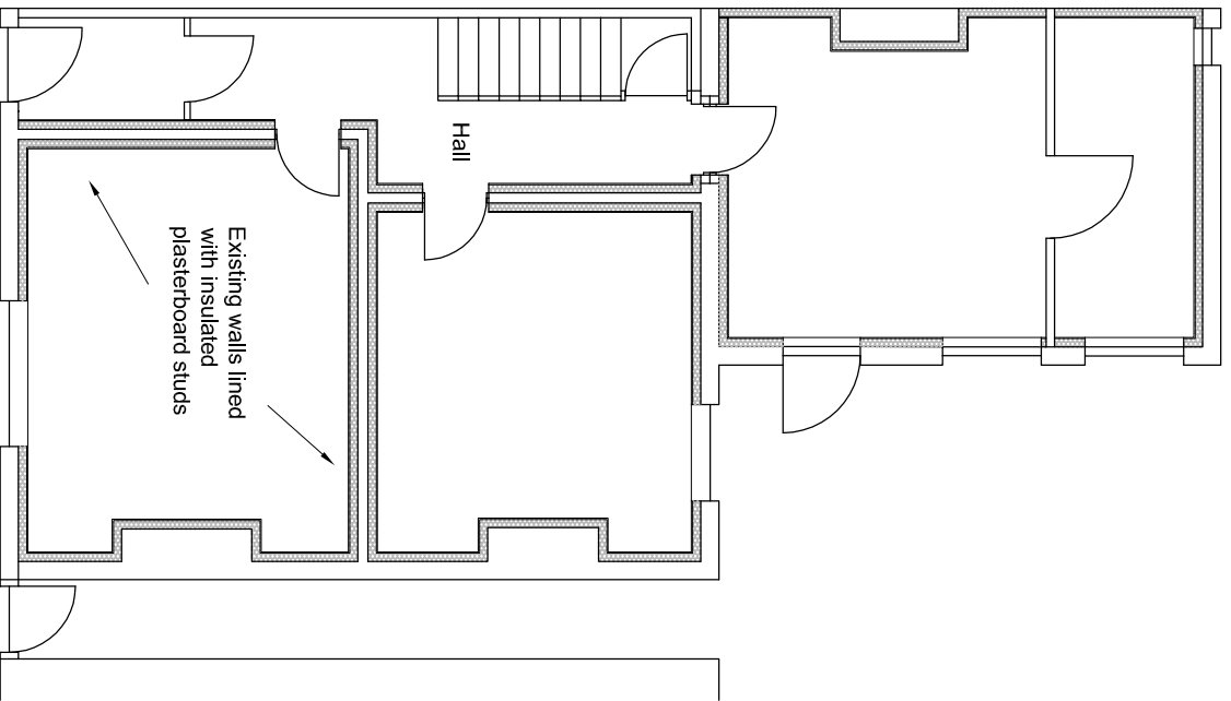
EXISTING GROUND FLOOR LAYOUT (scale 1:100)
