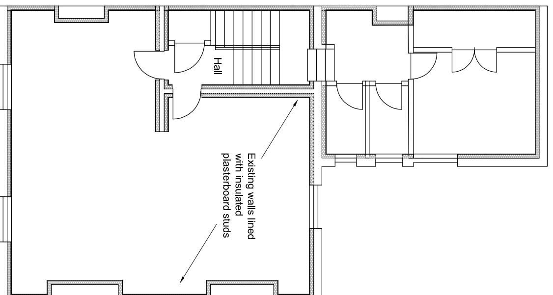
EXISTING FIRST FLOOR LAYOUT (scale 1:100)
