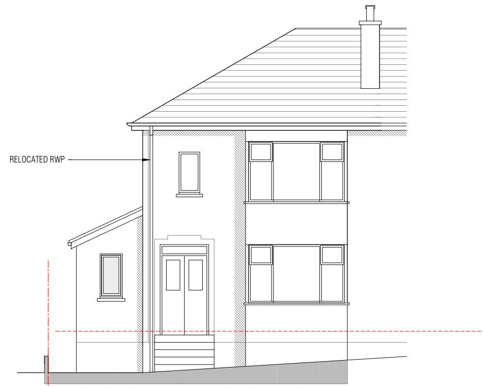
NORTH ELEVATION
