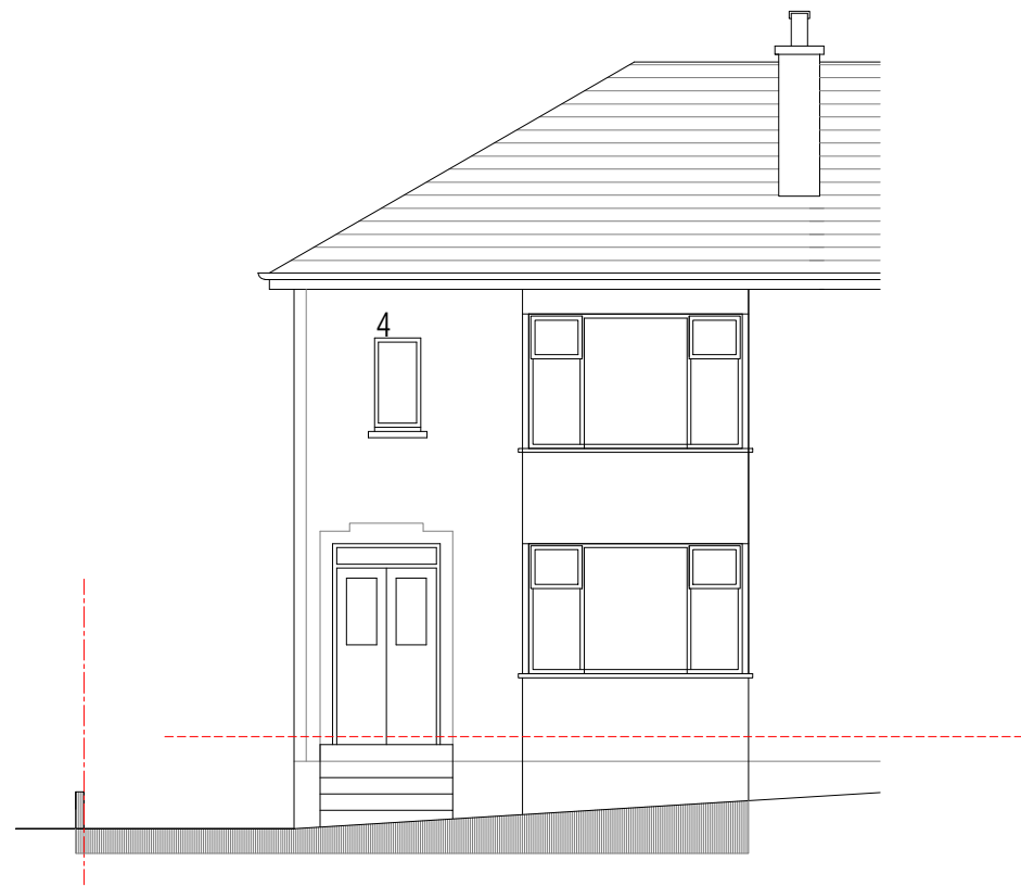
NORTH ELEVATION
