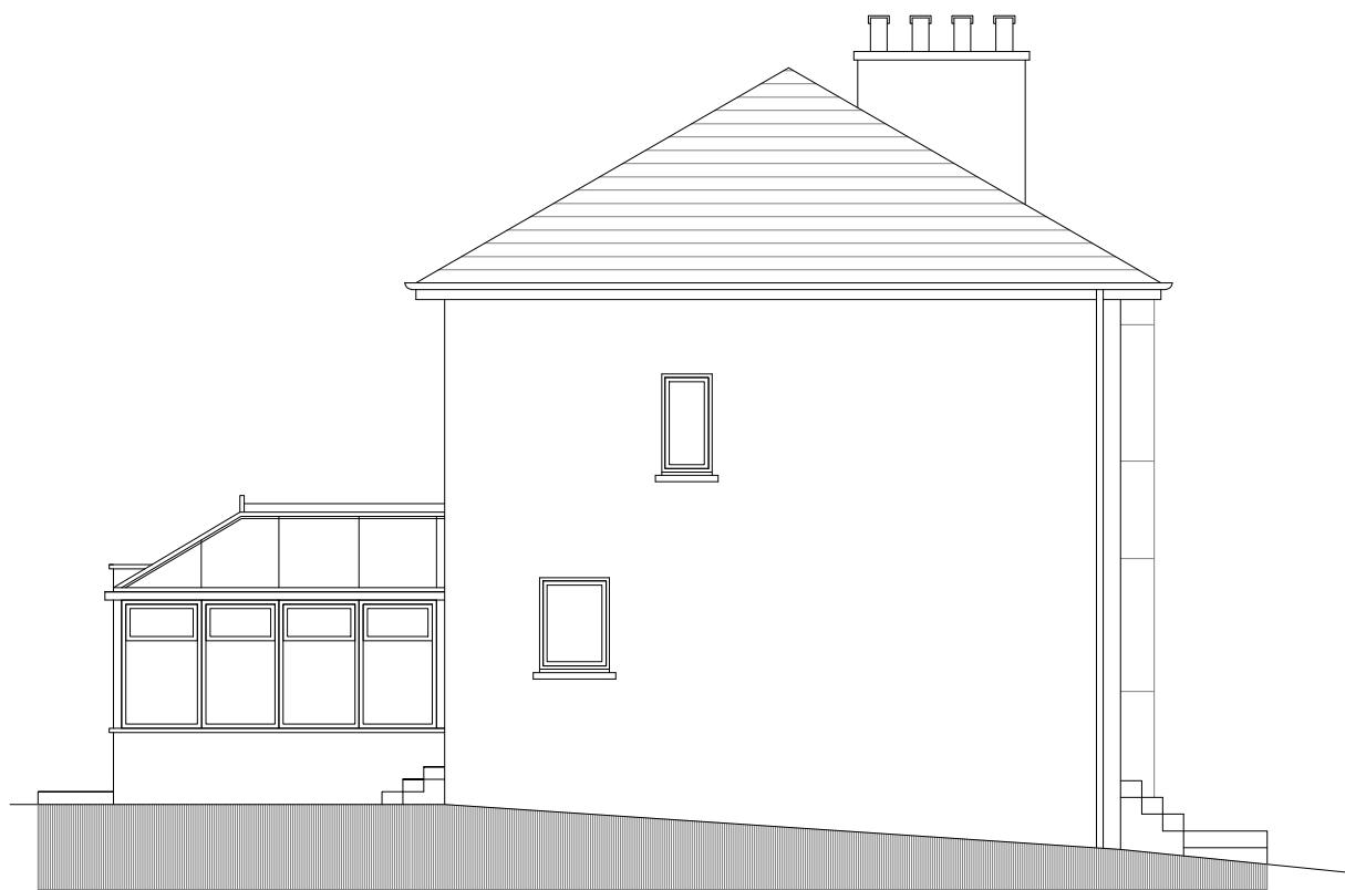
EAST ELEVATION
