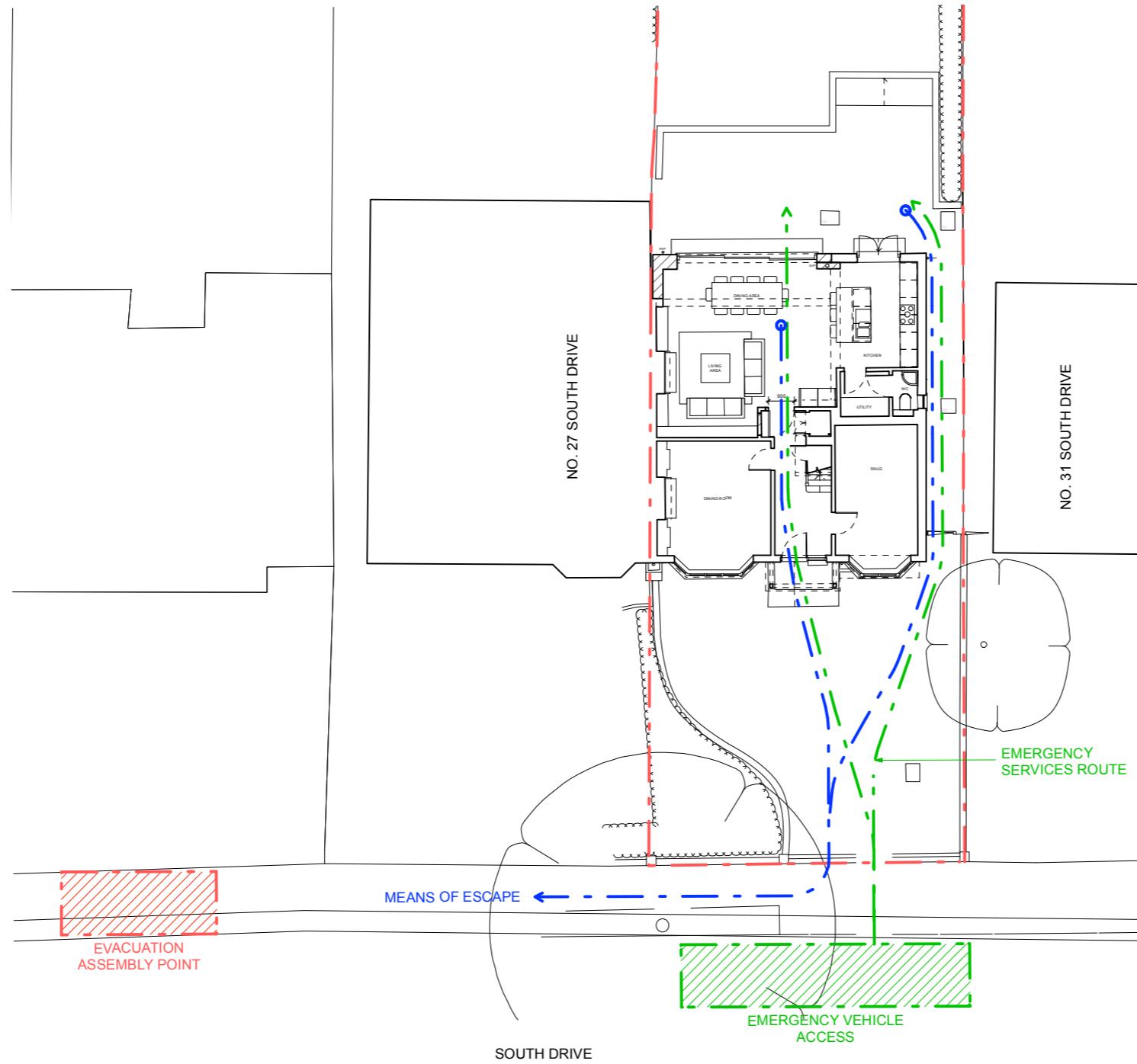
PROPOSED FIRE SAFETY STRATEGY PLAN 1:200
