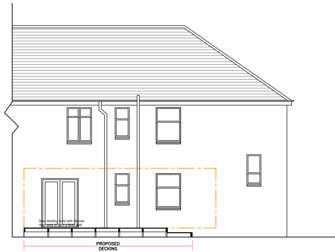
REAR ELEVATION SHOWING DECKING
