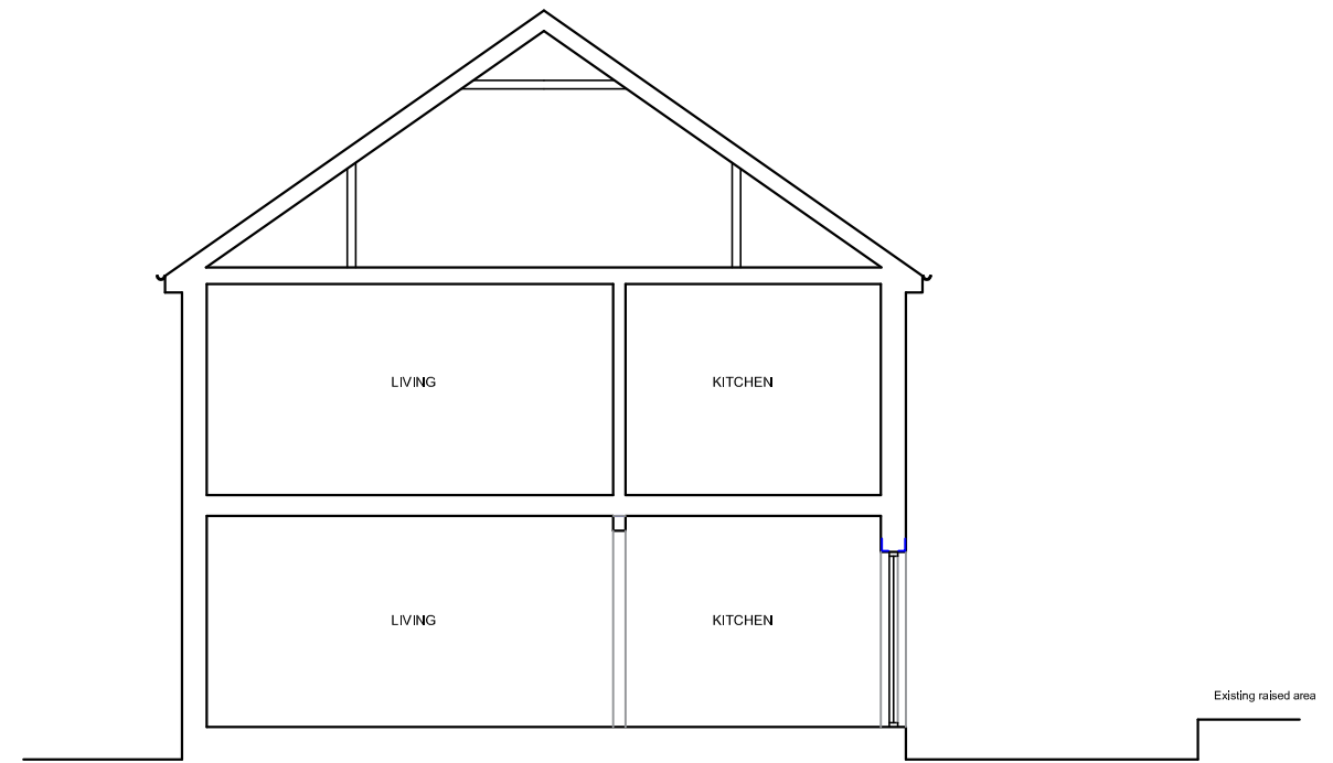
EXISTING SECTION
