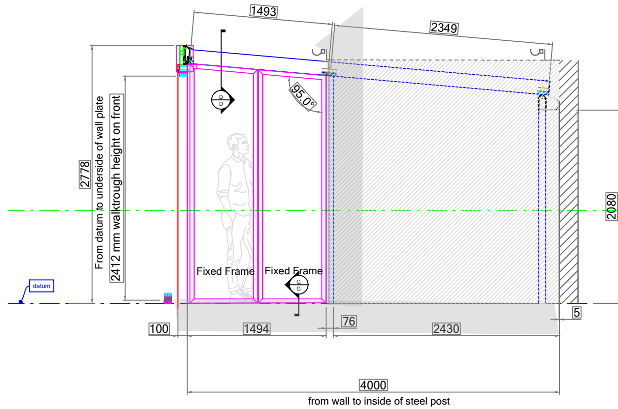
RHS Elevation (Viewed From Outside)
