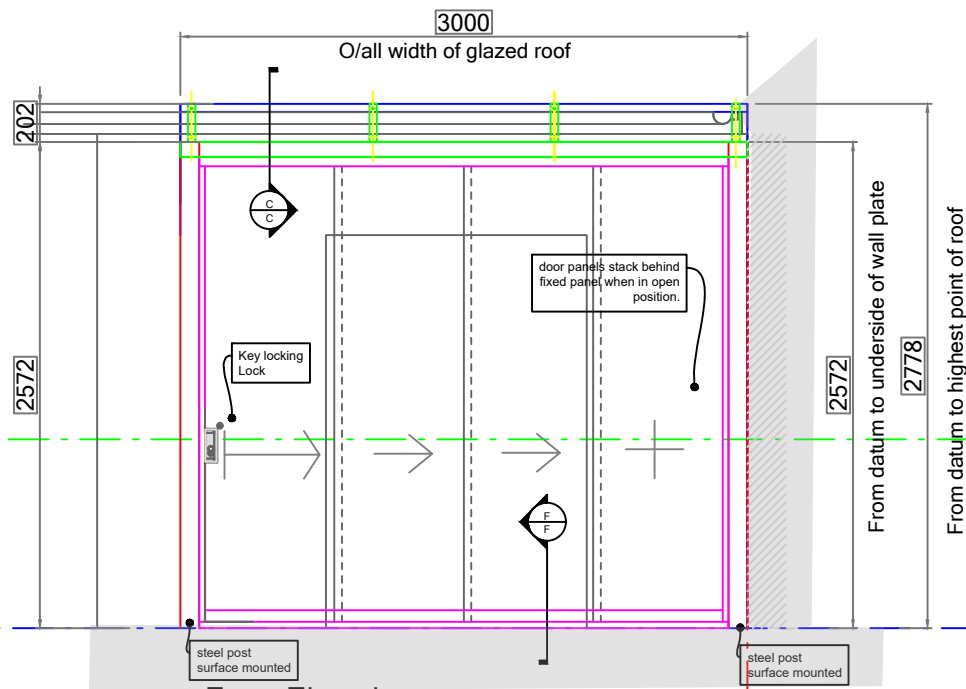
Front Elevation (Viewed From Outside)
