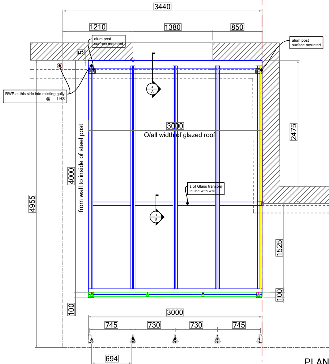
PLAN VIEW
