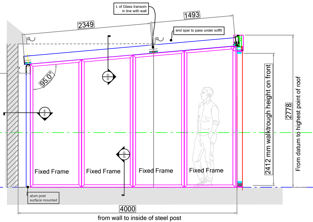
LHS Elevation (Viewed From Outside)
