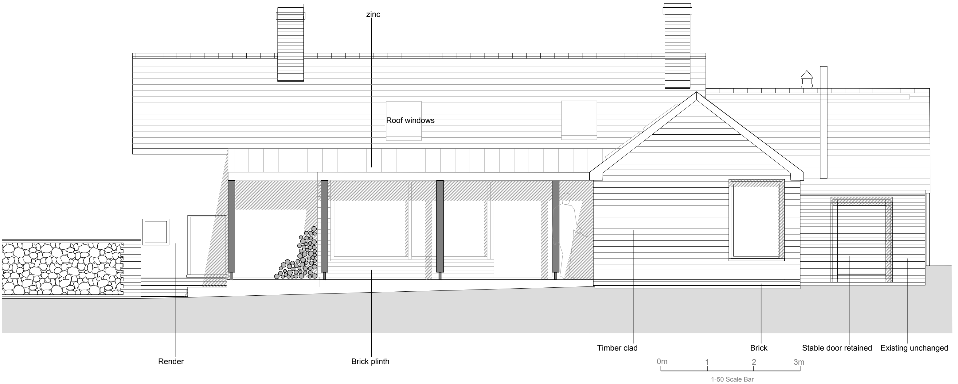
Proposed South Elevation SCALE 1-50@A3
