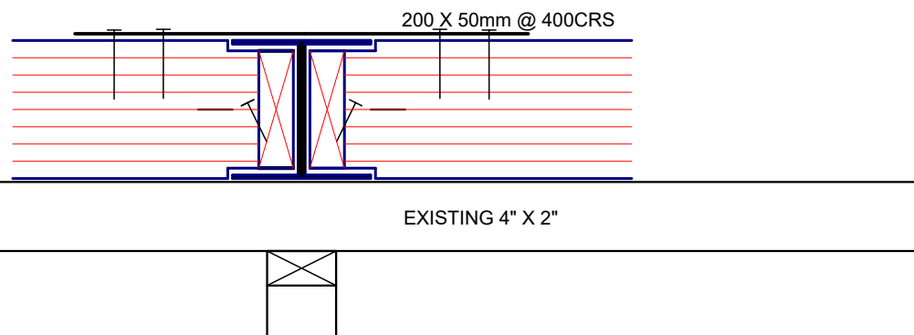
DETAIL 8
