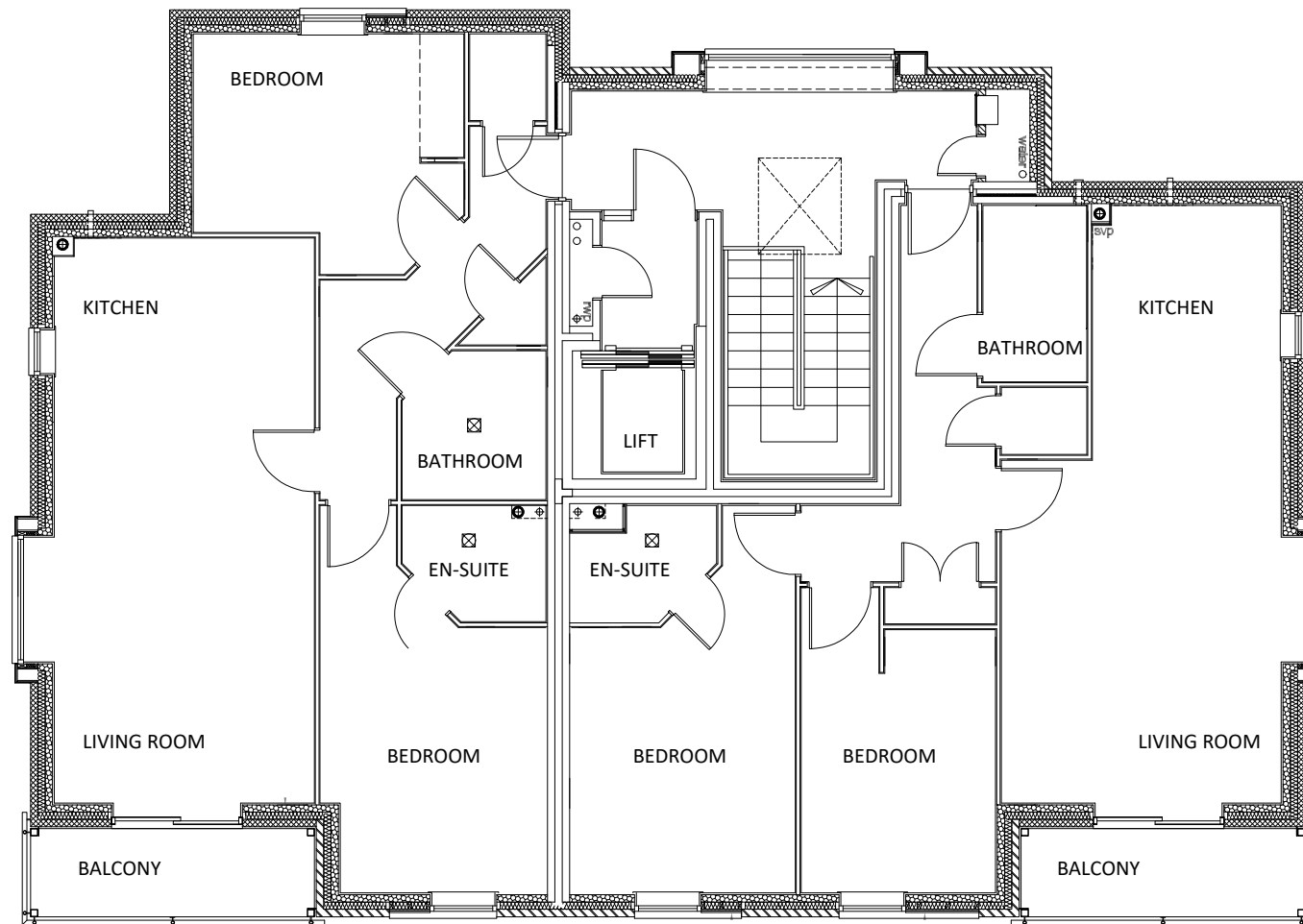
EXISTING FOURTH FLOOR
