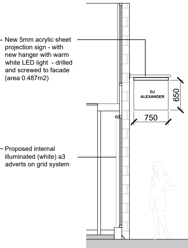
SECTION SCALE @ 1:50
