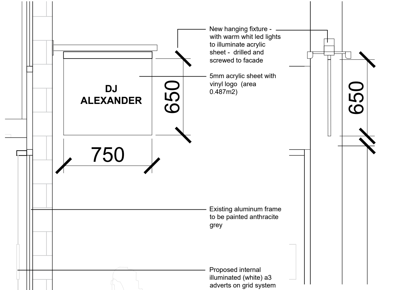
SECTION SCALE @ 1:20
