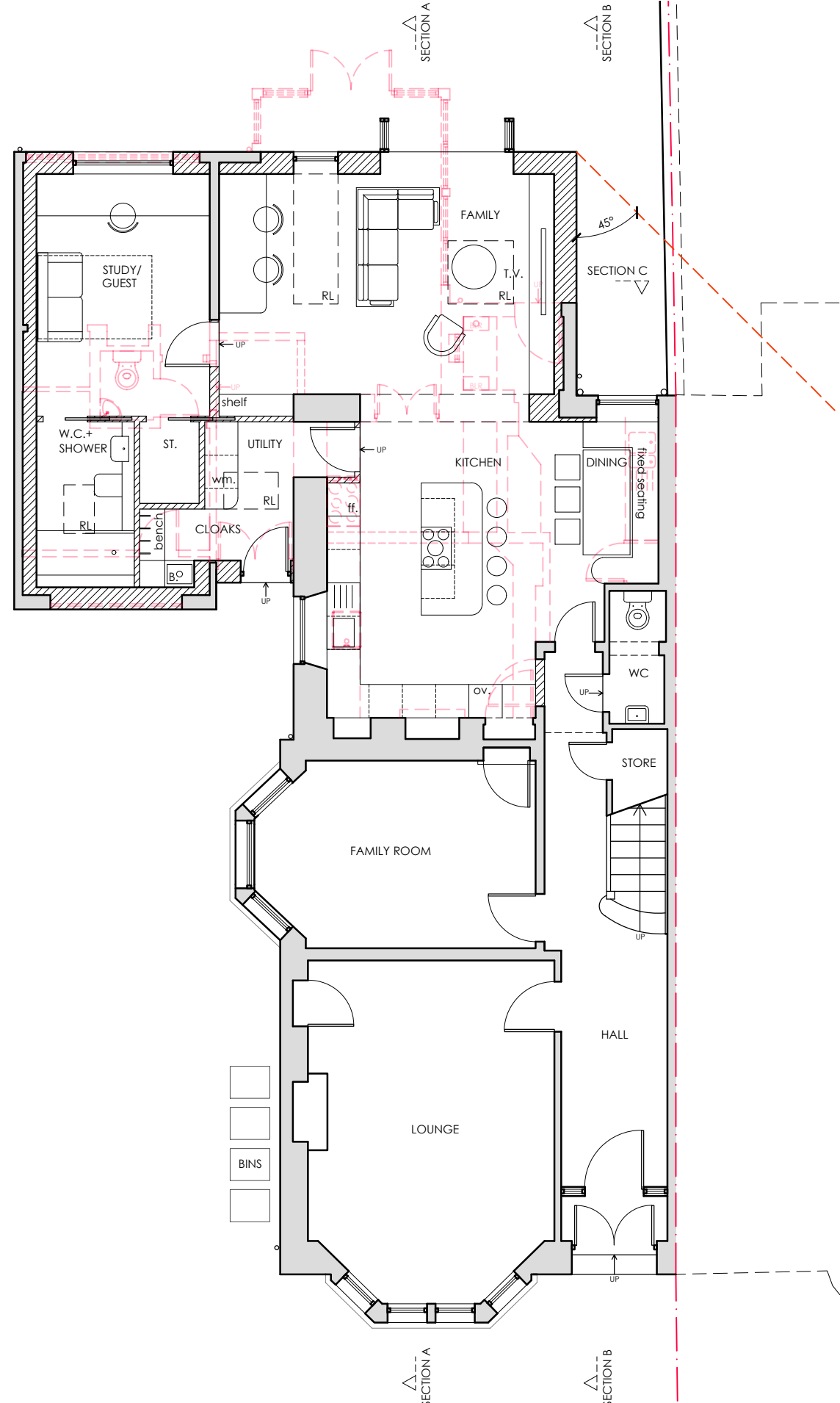
GROUND FLOOR PLAN AS PROPOSED - DOWNTAKINGS
