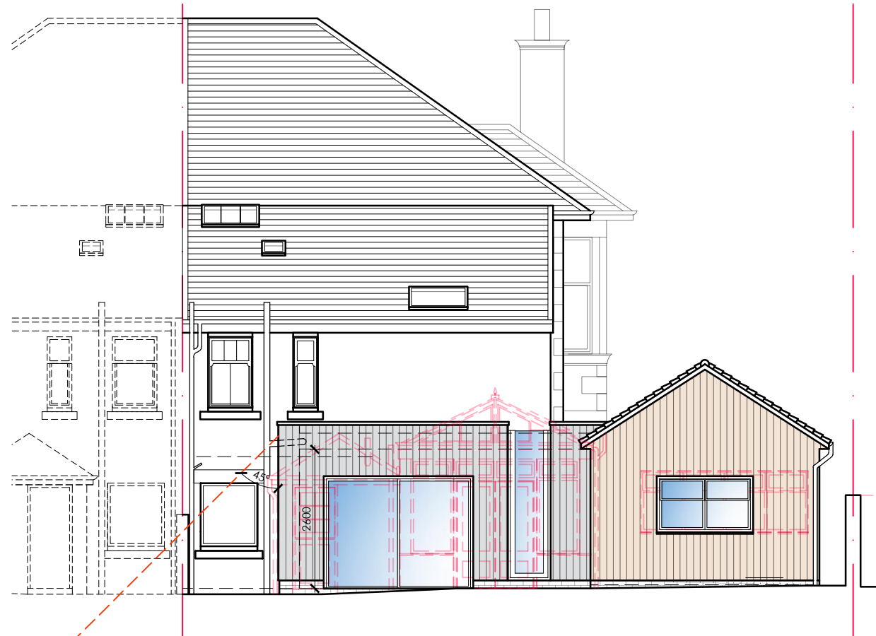
REAR ELEVATION AS PROPOSED - DOWNTAKINGS
