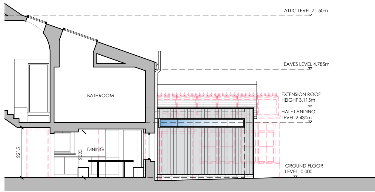
SECTION B-B AS PROPOSED - DOWNTAKINGS
